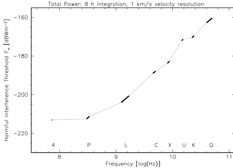
Figure 1: Calculated maximum acceptable power flux density (of an interfering signal) at different VLA bands, using typical observational values for the integration time (8 h) and the velocity resolution (1 km/s).
