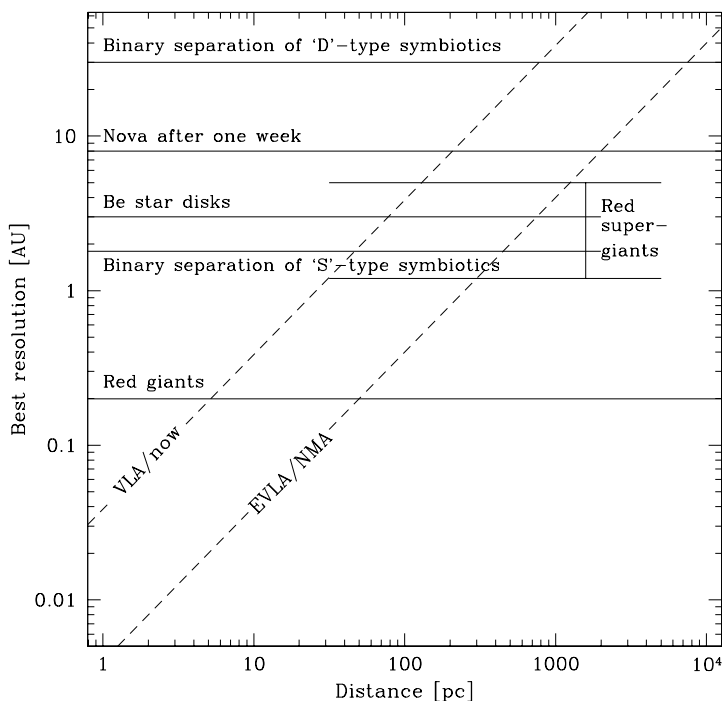
Figure B.11: The resolving power of the current and the expanded VLA (NMArray), compared to the linear dimensions of several known, thermal, radio-emitting astrophysical phenomena.
