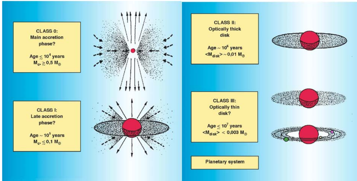
Figure B.4: In the current “standard model” of star formation, young stellar objects (YSOs) are divided into classes based on their spectral energy distributions. In the earliest stage of star formation, where most of the accretion takes place, the emission from Class 0 sources is completely dominated by far infrared emission from cold dust. In all cases the source also hosts a thermal jet, indicating the fundamental role of such outflows in the star formation process. In the next stage, Class I sources are less uniformly surrounded by dust; much of the accreting material is now in the form of a thin disk, and the observed emission is dominated by a combination of that from the star itself, and thermal emission from the disk and residual dust cloud. Class II sources are distinguished by the dominance of the stellar black body and the near disappearance of the dust cloud. Finally, Class III sources host a much less massive (and optically thin) disk, and may start to form planets.
