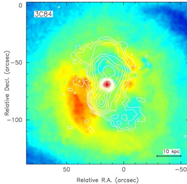
Figure 3.15: The cooling core source 3C 84 in the Perseus galaxy cluster: 1.4 GHz (VLA) contours over 0.5–1 keV (Chandra) color image, from Fabian et al. (2000). Note the anti-correlation between the radio lobes and the X-ray emission, and the bright X-ray rims around the radio lobes. These rims are cooler than the surrounding gas, and not the result of shocks; the bubbles themselves may contain hotter gas. The radio-emitting plasma has pushed the X-ray emitting gas aside.
