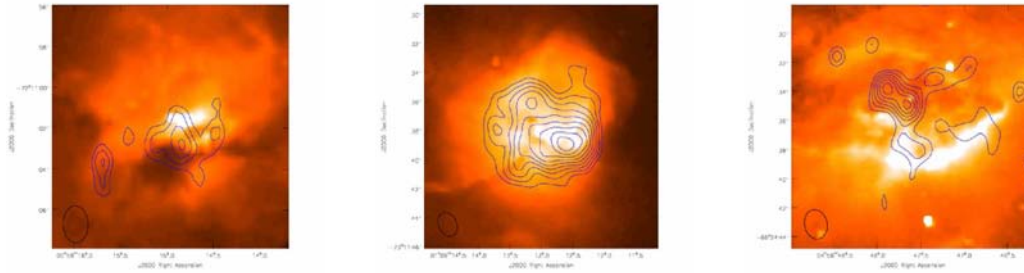
Figure 3.4: Three sample ultracompact H II regions in the Magellanic Clouds, as seen in H \alpha (from HST; color scale) and 8.4 GHz radio continuum emission (contours; from the Australia Telescope Compact Array). The linear resolution of the radio data is \sim 1 pc. Candidate regions were selected by their IRAS colors. The full EVLA will allow higher-resolution imaging of entire galaxies, out to the distance of NGC 253 (2.6 Mpc). From Indebetouw, Johnson, & Conti (submitted).
