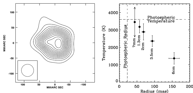
Figure B.10: ( left ) VLA 43 GHz image of Betelgeuse. The resolution is 40 milliarcseconds and the contour interval is 250 K (brightness temperature). ( right ) The variation of temperature in the atmosphere with radius, determined from the VLA observations of Betelgeuse at different frequencies which resolve the source size (Lim et al. 1998). The NMArray will give a factor \sim 10 higher resolution at 30 times higher sensitivity.
