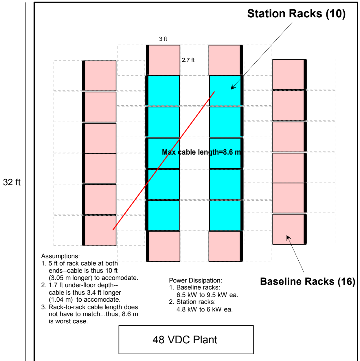
Figure 8-4 Preliminary 40-station correlator system floor-plan.
