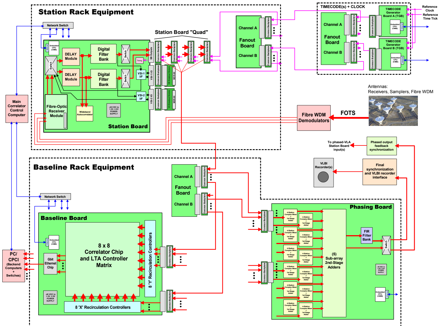
Figure 8-2 Correlator module connectivity diagram.
