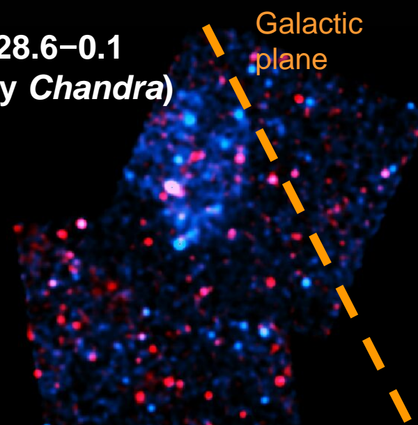
G32.45-0.1 (by XMM ) red: soft X-ray blue: hard X-ray
