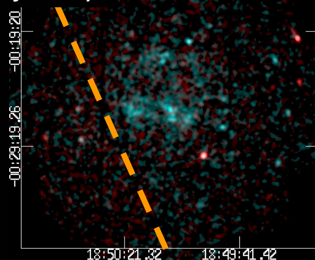
G32.45-0.1 (by XMM ) red: soft X-ray blue: hard X-ray
