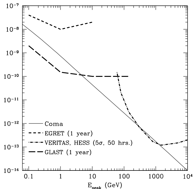
Figure 6: Predicted \gamma -ray emission from the Coma cluster of galaxies from the cluster merger shock model. The solid curve is the integrated number of particles per \text{cm}^2 per \text{s}^{-1} greater than E_{\text{peak}} . Observational limits for EGRET , GLAST , and VERITAS and HESS are included. The EGRET and predicted GLAST observational limits are 1 year integrations. The quoted VERITAS and HESS limits are 50 hour, 5\sigma limits (Weekes et al., 2002). The vertical axis represents the number of particles greater than E_{\text{peak}} in units of \text{cm}^{-2} \text{ s}^{-1} .
