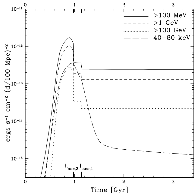
Figure 2: Same as Fig. 1 except light curves are given in energy flux at 40–80 keV, > 100 MeV, > 1 GeV and > 100 GeV. Curves are labeled in the diagram.
