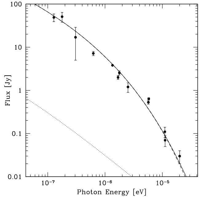
Figure 4: Comparison of radio observations of the Coma cluster with the cluster merger shock model. The solid curve is the total expected radio emission, the dashed curve is the contribution to the total emission from primary electrons, and the dotted curve from secondary electrons and positrons. The solid circles are observational data points taken from Thierbach, Klein & Wielebinski (2003).
