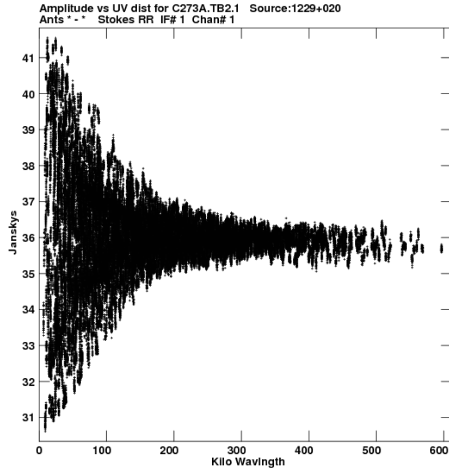
Visibility Amplitude
