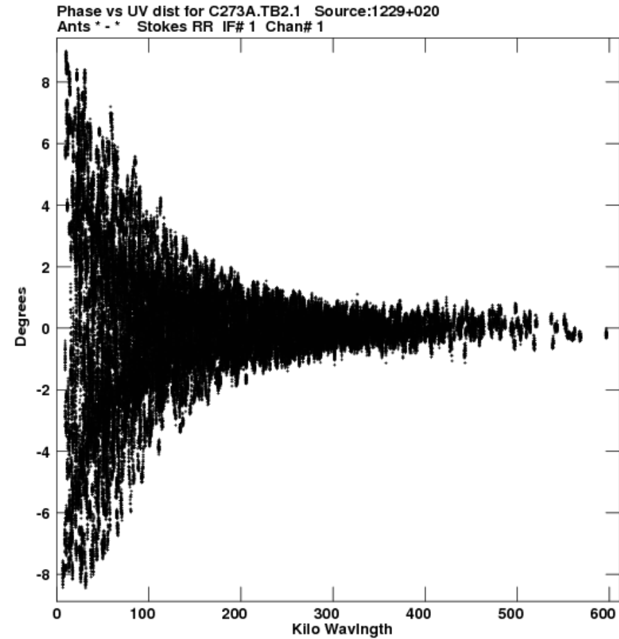
Visibility Phase
