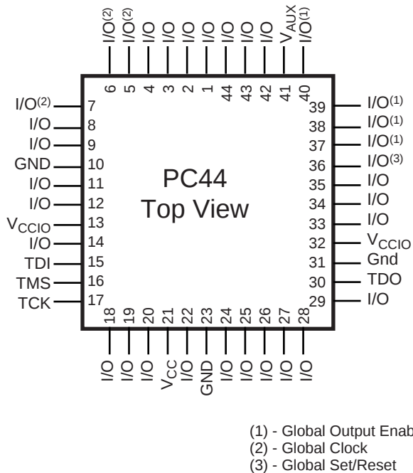
Figure 7: PC44 Package
