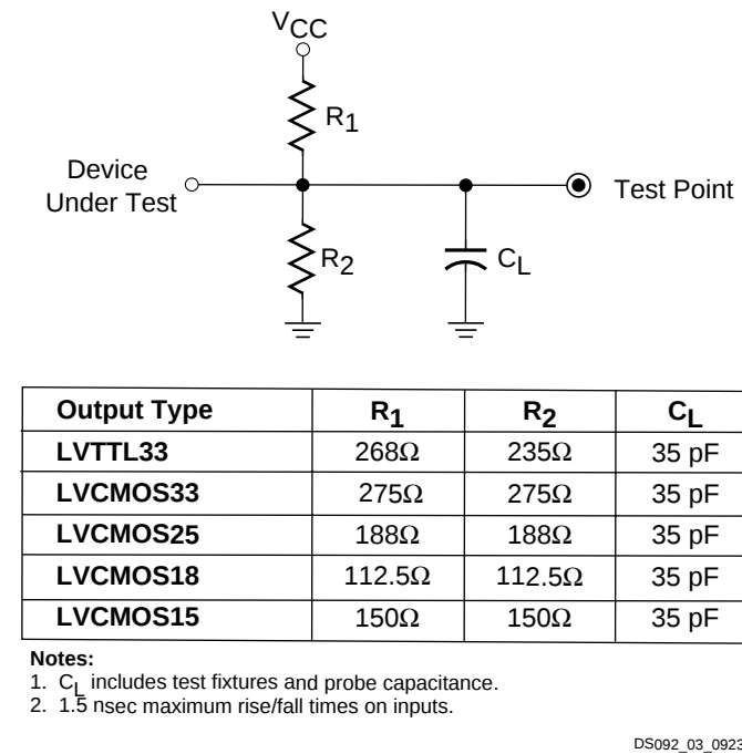
Figure 3: AC Load Circuit
