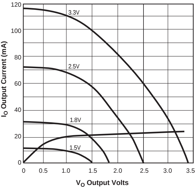
Figure 4: Typical I/O Output Curves
