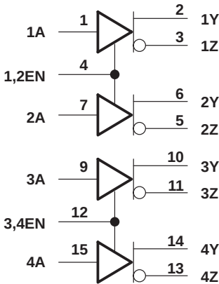
SN65LVDS3487 logic diagram (positive logic)
