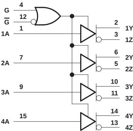
'LVDS31 logic diagram (positive logic)
