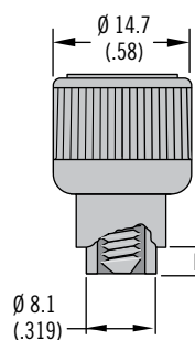
Flare-In Style
