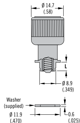
Floating Style
