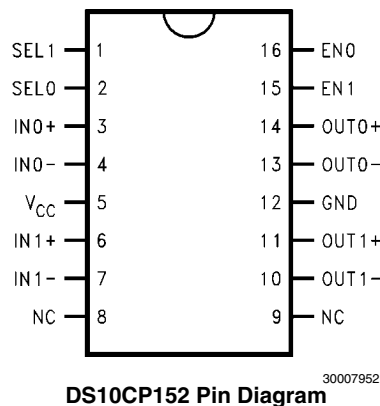
DS10CP152 Pin Diagram
