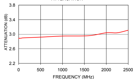
LAT-3+ ATTENUATION
