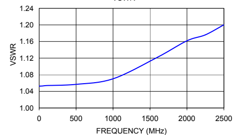
LAT-3+ VSWR
