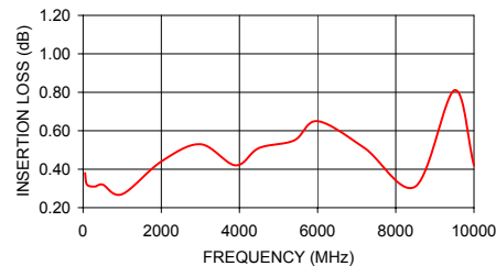
ADCH-80 INSERTION LOSS
