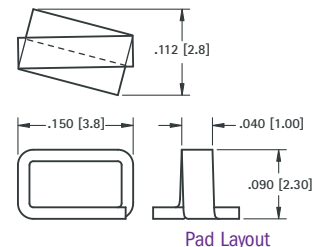
Pad Layout
