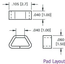
Pad Layout
