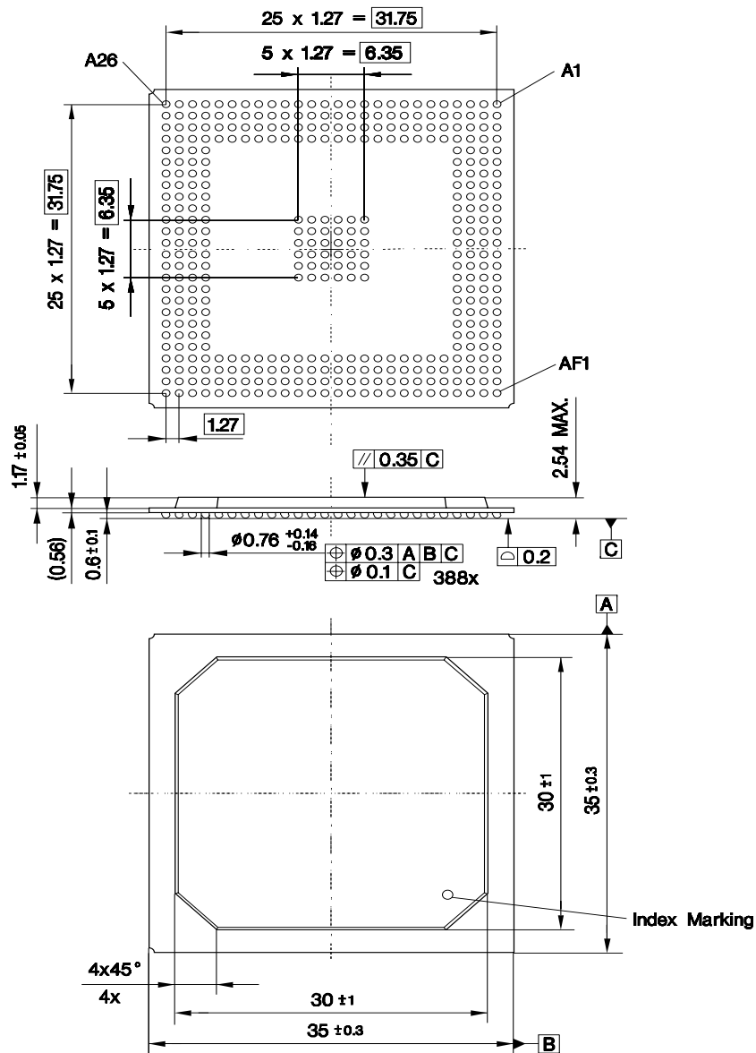
Figure 46 P-BGA-388-2 Package
