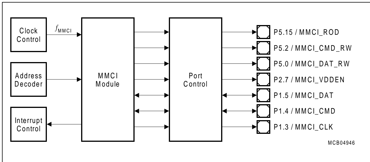
Figure 9 General Block Diagram of MMCI Interface
