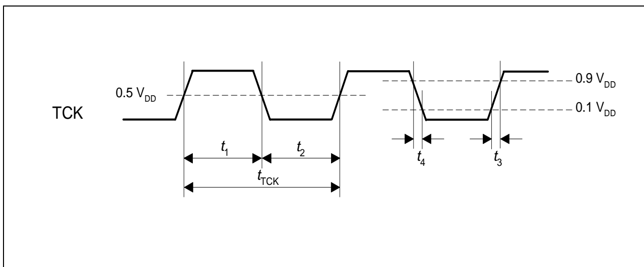
Figure 36 TCK Clock Timing
