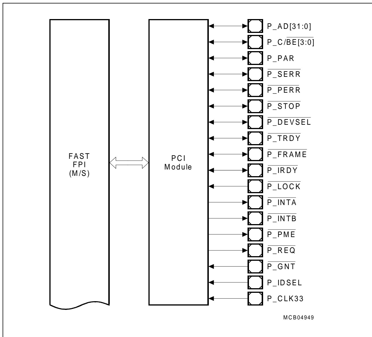
Figure 11 General Block Diagram of the PCI Interface
