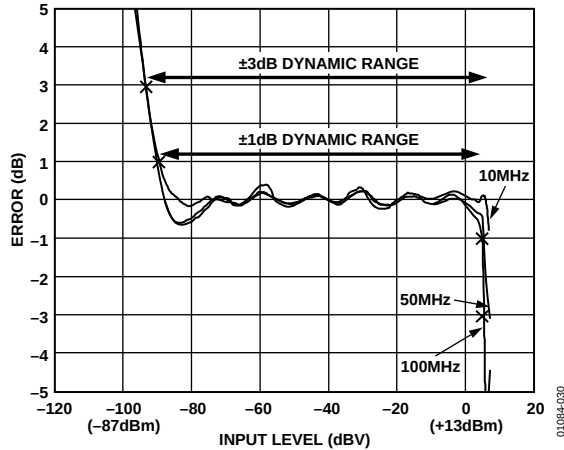
Figure 30. Log Conformance Error vs. Input Level at 10 MHz, 50 MHz, and 100 MHz
