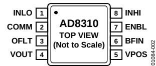
Figure 2. Pin Configuration
