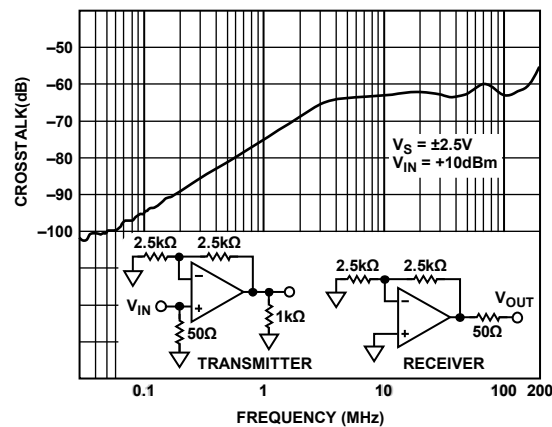
Figure 42. Crosstalk vs. Frequency
