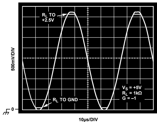
Figure 38. Output Swing
