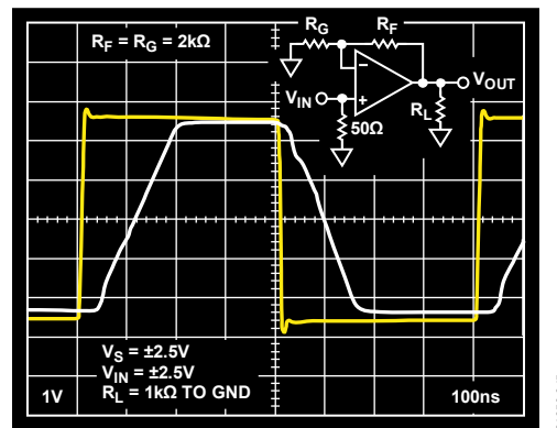
Figure 45. Overdrive Recovery
