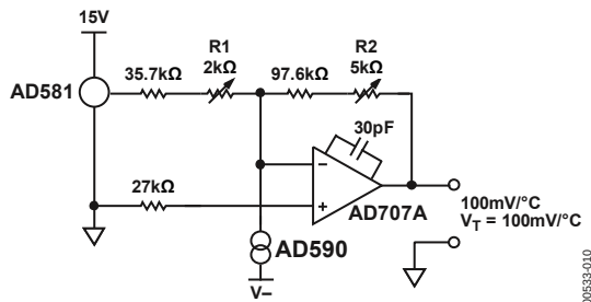
Figure 12. 2-Temperature Trim
