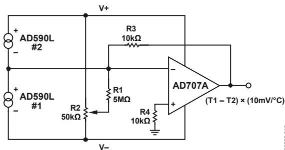
Figure 18. Differential Measurements
