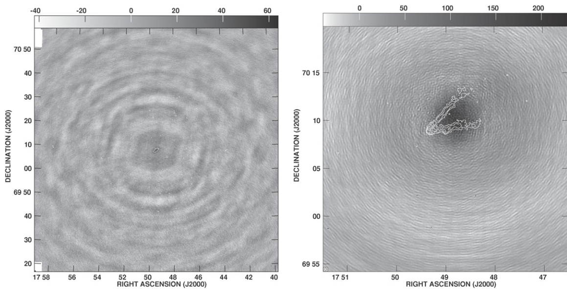
Figure 16. In grayscale, the multi-scale Clean image minus point-source Clean image of (left) the continuum emission and (right) the H I line emission at V = 98.3 \text{ km s}^{-1} in NGC 6503. The grayscale ranges are shown in the step wedges, labeled in \mu\text{Jy} . The multi-scale images in the continuum and the H I are sketched in with contours. The Clean beam is illustrated at the lower left corner in both images and is nearly invisible on these scales.
