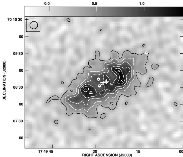
Figure 2. 21 cm radio continuum distribution in NGC 6503. The wedge at the top shows the displayed brightness in mJy beam -1 , and the contours are drawn at (1, 2, 3, 4, 5) × 0.25 mJy beam -1 . The Clean beam is plotted in the top left corner. The continuum peaks are marked by crosses, the six unresolved X-ray sources found by Lira et al. (2007) are marked by stars, and the kinematic center of the H I distribution (Section 4.2) is marked by a plus sign.
