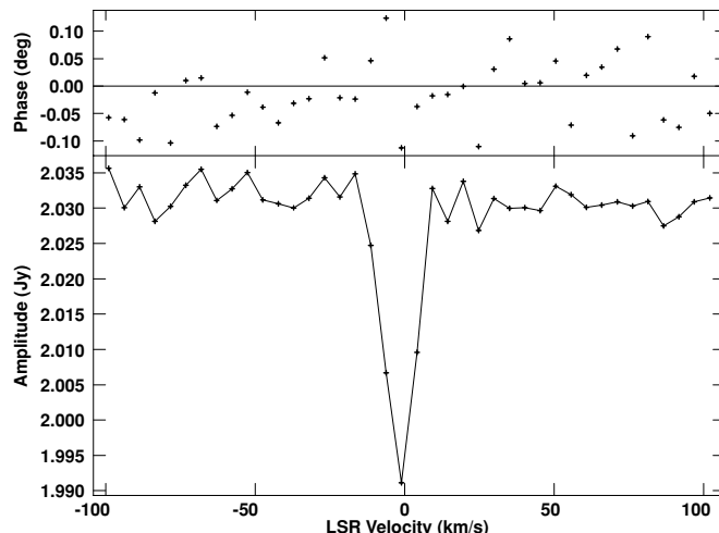
Figure 6. Spectrum of calibration source 1800+784 computed by vector averaging all calibrated fringe visibilities.
