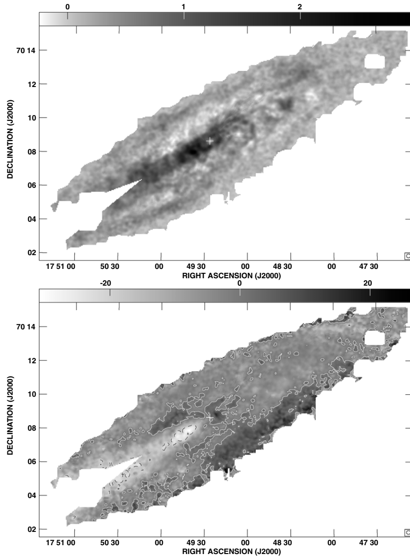
Figure 13. Top: zeroth-moment image of NGC 6503 minus that fit by CUBIT plotted with a logarithmic grayscale. The step wedge is marked in steps of 10^{21} \text{ cm}^{-2} . A comparison of the CUBIT model and the radial column density along the major axis is shown in Figure 14. Bottom: first-moment image of NGC 6503 minus that fit by CUBIT. The white contour is drawn at 0 \text{ km s}^{-1} , and the black, dashed contour is drawn at -20 \text{ km s}^{-1} .
