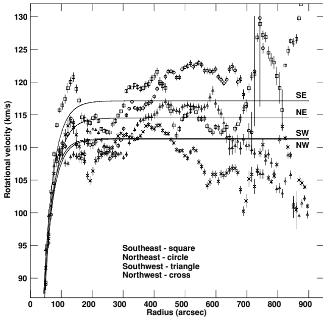
Figure 12. Rotation curve fit by the GAL program for the NW (cross symbols), SW (triangles), NE (circles), and SE (squares) quadrants. Note that the velocity tick marks are separated by about one spectral channel in this blown-up display.
