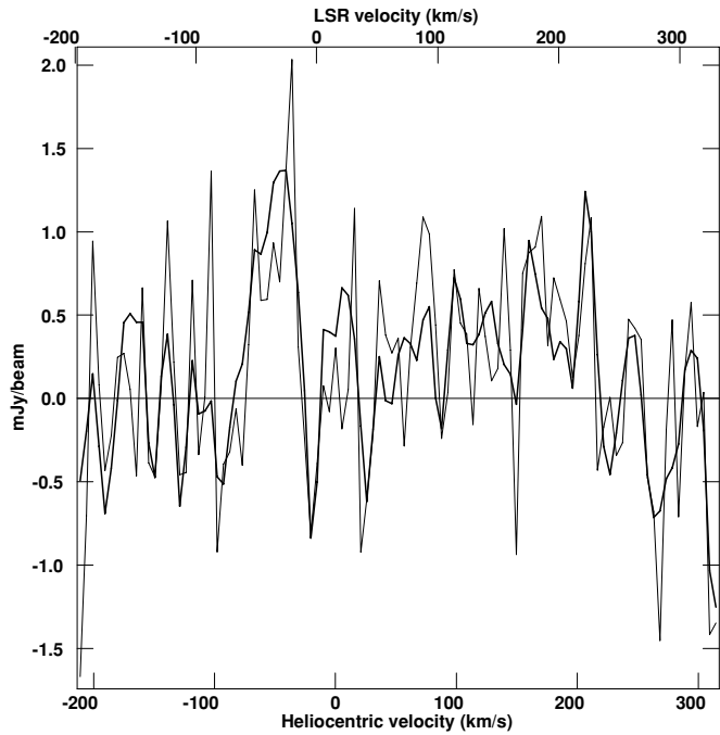
Figure 7. Spectrum at the position of 1748+700 (R.A. = 17^{\text{h}}48^{\text{m}}32^{\text{s}}.84 , decl. = +70^{\circ}05'50''.8 in J2000) minus the measured continuum flux density of 755 mJy. The light line from the high-resolution, primary-beam-corrected data cube (rms = 0.58 \text{ mJy beam}^{-1} ). The heavy line from a version of the data cube smoothed to 30'' spatial resolution and 10 \text{ km s}^{-1} velocity resolution (rms = 0.38 \text{ mJy beam}^{-1} ).
