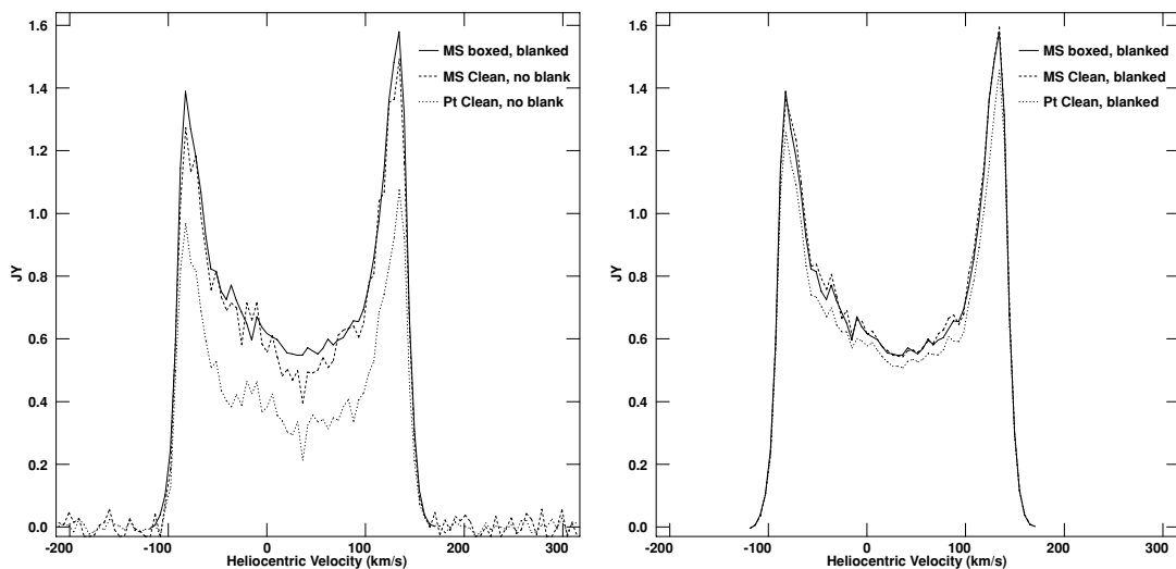
Figure 17. Primary-beam-corrected integrated spectrum of NGC 6503 obtained using a number of Cleaning and blanking prescriptions. Left: the solid line is the integral over the blanked cube, made from a carefully boxed Clean of each channel image (reproduced from Figure 10). The dashed line is the integrated spectrum over a rectangular region slightly larger than the extent of the zeroth-moment image constructed with multi-scale Clean with little restriction of the Cleaning area. The dotted line is the integrated spectrum constructed in the same way but using only point-source Clean components. Right: Same as left, but only unblanked regions in the carefully boxed cube are included in each profile.
