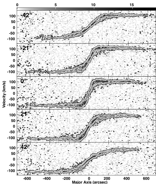
Figure 4. Primary-beam-corrected images for slices parallel to the major axis, separated by 21". Axis labels are relative to the kinematic center and the systemic velocity. The grayscale is plotted from 0.5 to 18.65 mJy beam -1 with a logarithmic transfer function and contours are plotted at 1.5, 3, 6, and 12 mJy beam -1 .
