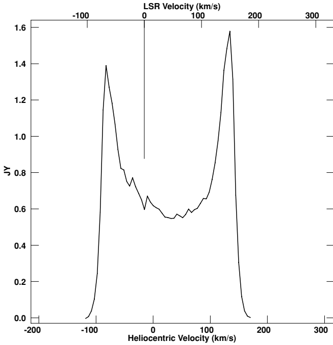
Figure 10. Integrated spectrum of NGC 6503 after primary beam correction and blanking of line-free regions. The LSR as well as heliocentric velocities are shown, with a long tick mark at 0 \text{ km s}^{-1} LSR. Errors in the spectrum due to H I emission from the Milky Way are evident near this velocity.
