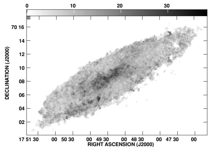
Figure 9. Second moment of the H I distribution in NGC 6503 plotted with a linear grayscale from 0 to 39 \text{ km s}^{-1} . No correction for projection effects has been made.
