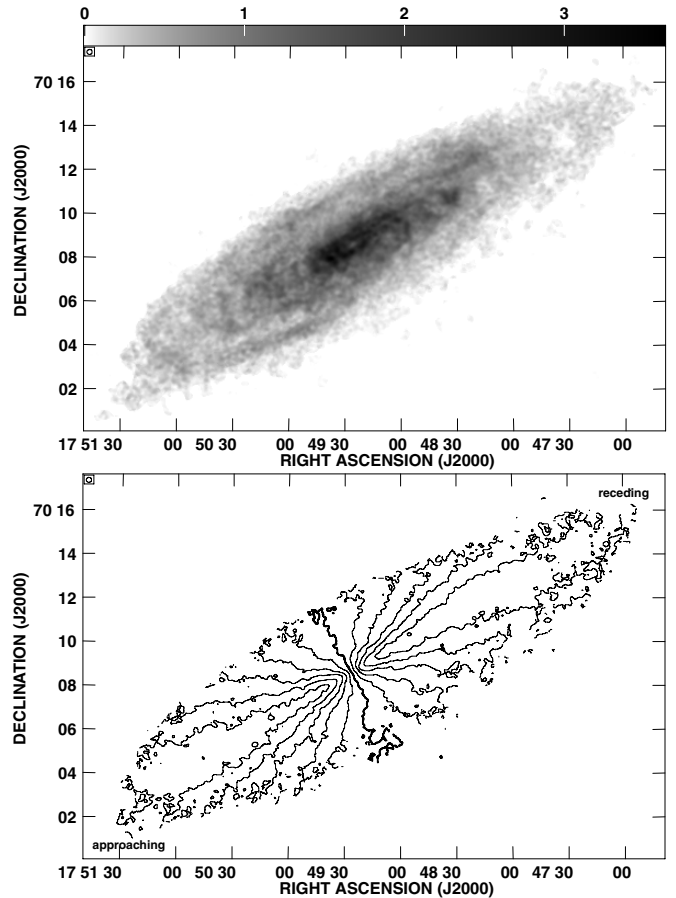
Figure 8. Top: zeroth moment of the H I distribution in NGC 6503 measured in 10^{21} \text{ cm}^{-2} and plotted with a logarithmic grayscale. The column density is 0.57 \times 10^{19} \text{ cm}^{-2} SdV , with SdV in units of \text{Jy beam}^{-1} \text{ m s}^{-1} . The lowest reliable H I emission from NGC 6503 is at 1.8 \times 10^{19} \text{ cm}^{-2} . Bottom: first moment of the H I distribution in NGC 6503. The heavy contour is plotted at 26 \text{ km s}^{-1} heliocentric (nearly the systemic velocity), and the other contours are spaced at 20 \text{ km s}^{-1} relative to this value. The eastern (E) side is approaching, while the western (W) side is receding.
