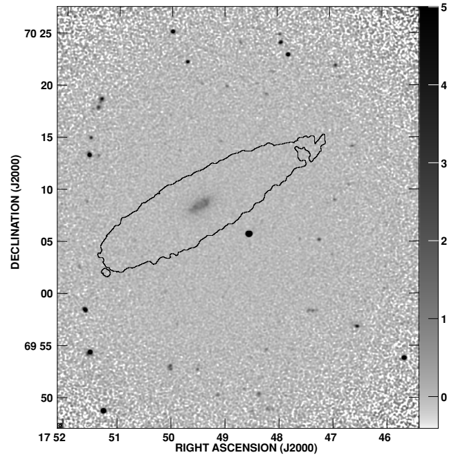
Figure 1. Primary-beam-corrected continuum image of a field near NGC 6503. The wedge to the right shows the displayed brightness in mJy beam -1 which is clipped at 5 mJy beam -1 . The extent of the detected H I emission is shown by the solid line (see Section 4.1). The quasar 1748+700 is the strong point source 5'.34 to the southwest (SW) of the galaxy.
