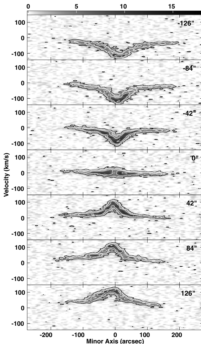
Figure 5. Primary-beam-corrected images for slices parallel to the minor axis, separated by 42". The axis labels are relative to the kinematic center and the systemic velocity. The grayscale is plotted from 0.5 to 18.65 mJy beam -1 with a logarithmic transfer function and contours are plotted at 1.5, 3, 6, and 12 mJy beam -1 .
