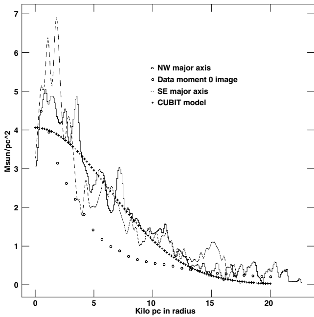
Figure 14. Radial column density in M_{\odot} \text{pc}^{-2} plotted against radius in NGC 6503. The plus signs trace the CUBIT model, the circles are averages over concentric rings in the zeroth-moment image, and the dashed and solid lines are slices in the zeroth-moment image along the major axis to the SE and NW, respectively. The slices have been corrected to radial column densities by multiplying by the cosine of the inclination ( 75^{\circ} :1).
