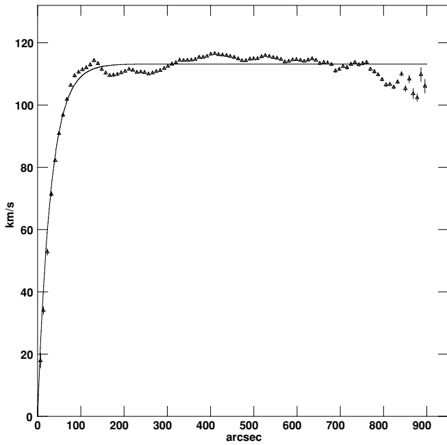
Figure 11. Rotation curve for the H I disk of NGC 6503, obtained from the AIPS program GAL by fitting all points in the first-moment image.
